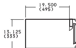
SNORKEL OVEN CAVITY DIMENSIONS USABLE WIDTH (NOT SHOWN) 26.250 (667) USABLE DEPTH 19.500 (495) USABLE HEIGHT 13.125 (333)
